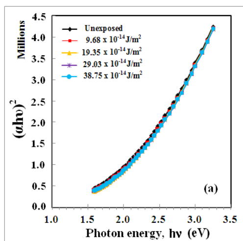
Fig.10. Plots of (\alpha h\nu)^2 against photon energy for chitosan powder before and after exposure to UV-ozone.
