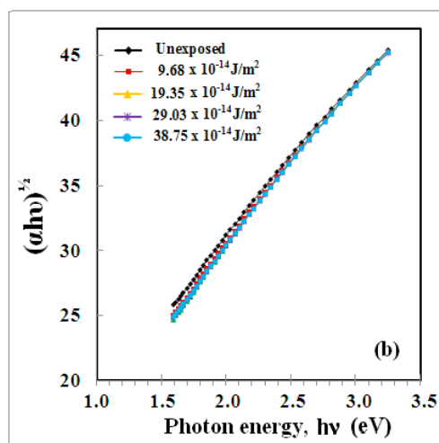
Fig. 11. Plots of (\alpha h\nu)^{1/2} against photon energy for chitosan powder before and after exposure to UV-ozone.
