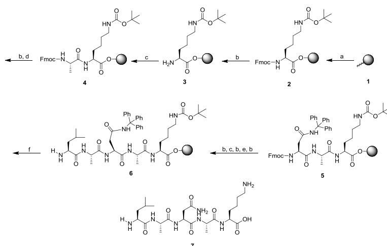
Scheme 1. Synthetic route of SCAP1. (a) (1) Fmoc-Lys(Boc)-OH, DIPEA, dichloromethane, 24 h, rt, (2) methanol: dichloromethane: DIPEA (15:80:5), 10 min, rt; (b) 20% piperidine in DMF; (c) Fmoc-Ala-OH, HOAt, HATU, DIPEA, dichloromethane:DMF (1:1), 4 h, rt; (d) Fmoc-Asn(Trt)-OH, HOAt, HATU, DIPEA, dichloromethane:DMF (1:1), 4 h, rt; (e) Fmoc-Leu-OH, HOAt, HATU, DIPEA, dichloromethane:DMF (1:1), 4 h, rt; (f) Trifluoroacetic acid 95% in water.
