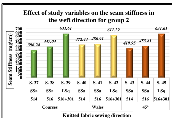
Figure 21: Effect of study variables on the seam stiffness in the weft direction for group 2
