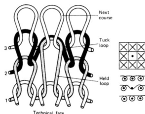
Figure 1: Show tuck stitch (13)
