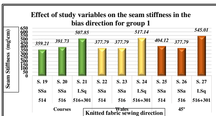
Figure 10: Effect of study variables on the seam stiffness in the bias direction for group 1
