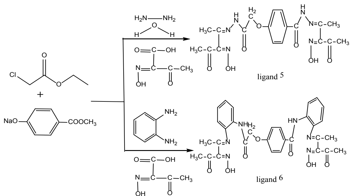
Scheme.3 Synthesis of ligands (5, 6)
