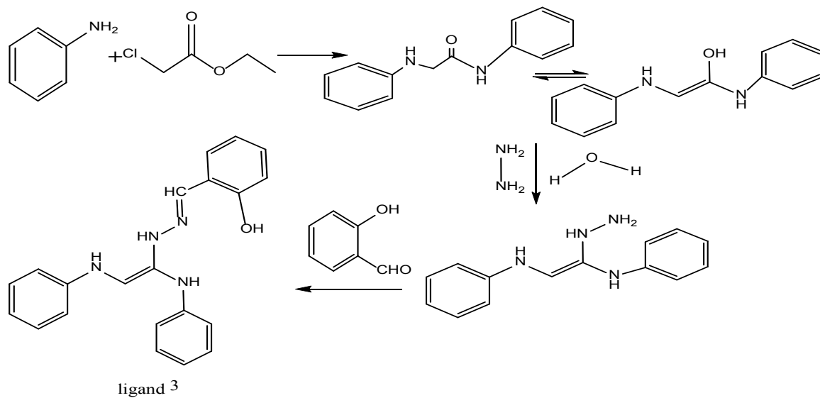
Scheme.2 Synthesis of ligand (3)
