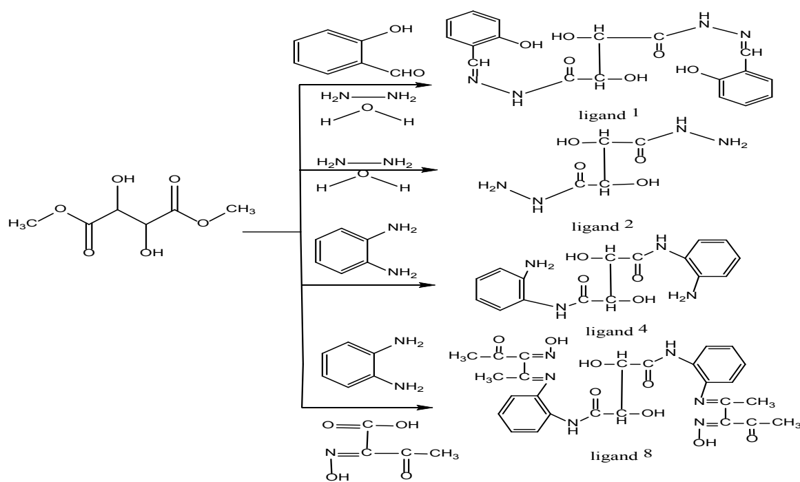
Scheme.1: Synthesis of ligands (1, 2, 4 and 8)
