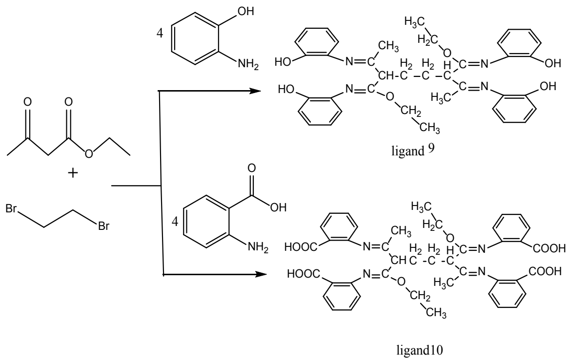
Scheme.5 Synthesis of ligands (9, 10)
