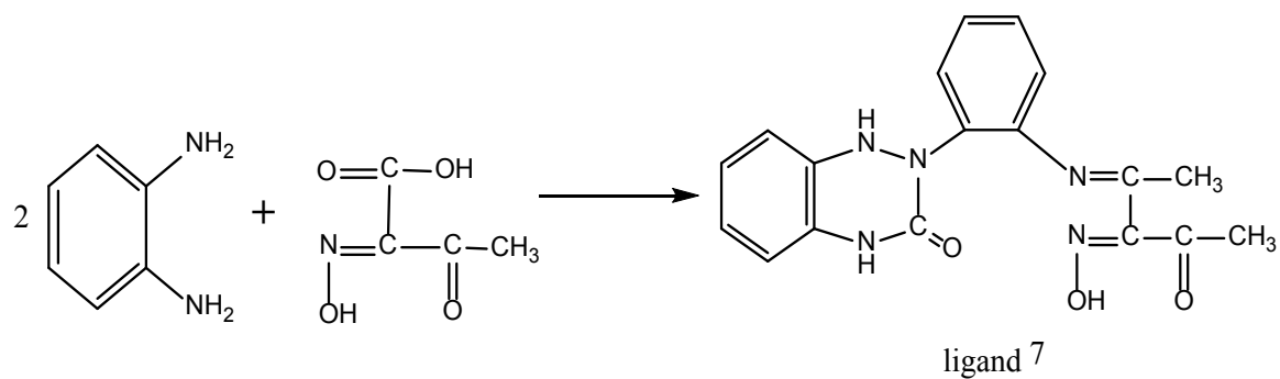
Scheme.4 Synthesis of ligand (7)
