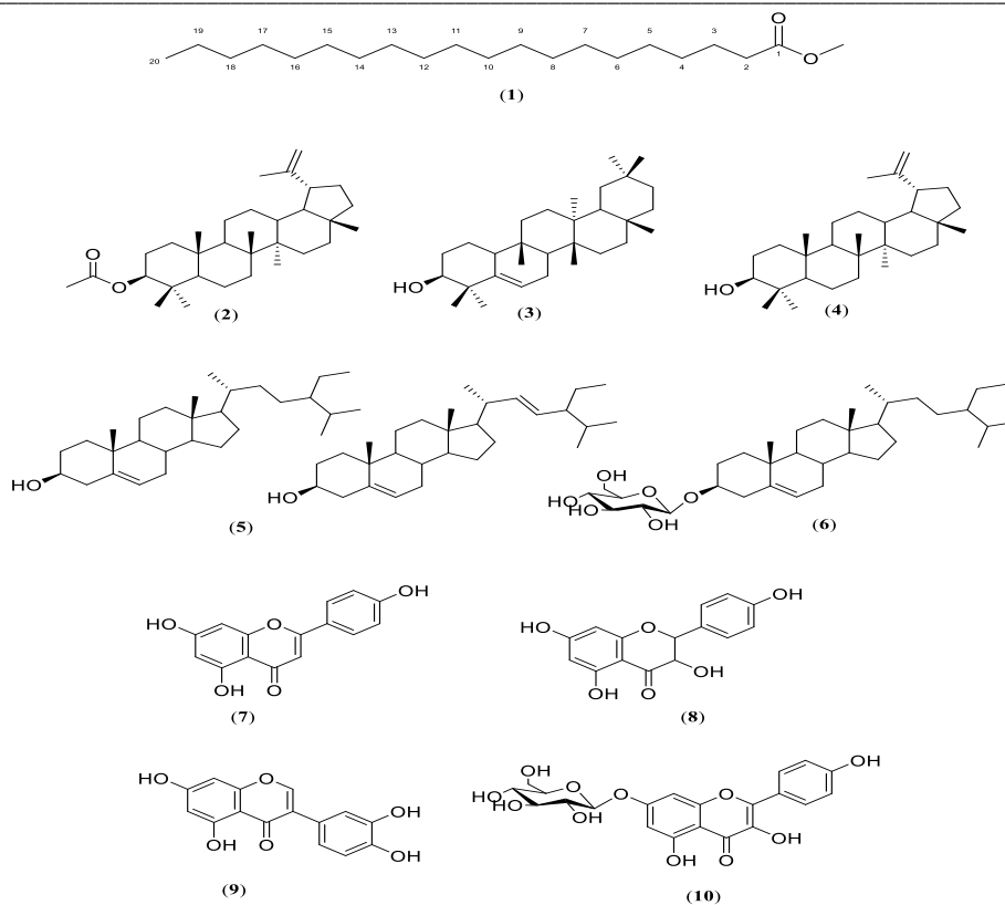
Fig. 1: Chemical structure of isolated compounds from M. spinosa
