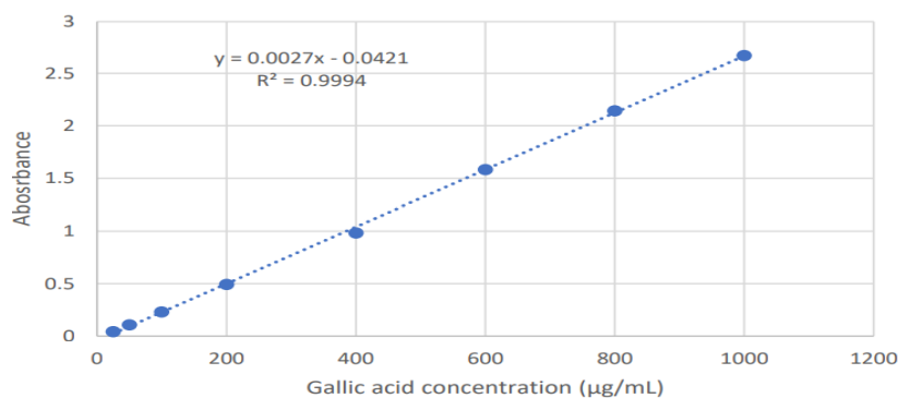
Fig. 2: Gallic acid standard calibration curve
