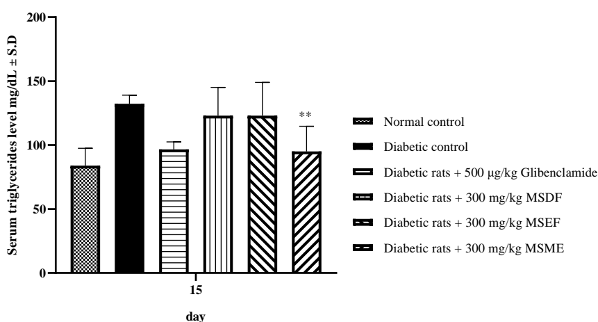
Fig 9: Effect of DCM (MSDF) and EtOAc (MSEF) fractions in addition to M. spinosa total methanolic extract (MSTME) on serum triglycerides level in STZ-induced diabetic rats. Columns represent mean \pm SD. A significant difference ( *p < 0.05 , **p < 0.01 , ***p < 0.001 ) when compared to diabetic control (one-way ANOVA followed by Tukey's test for multiple comparisons)
