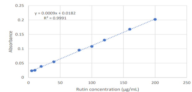
Fig. 3: Rutin standard calibration curve
