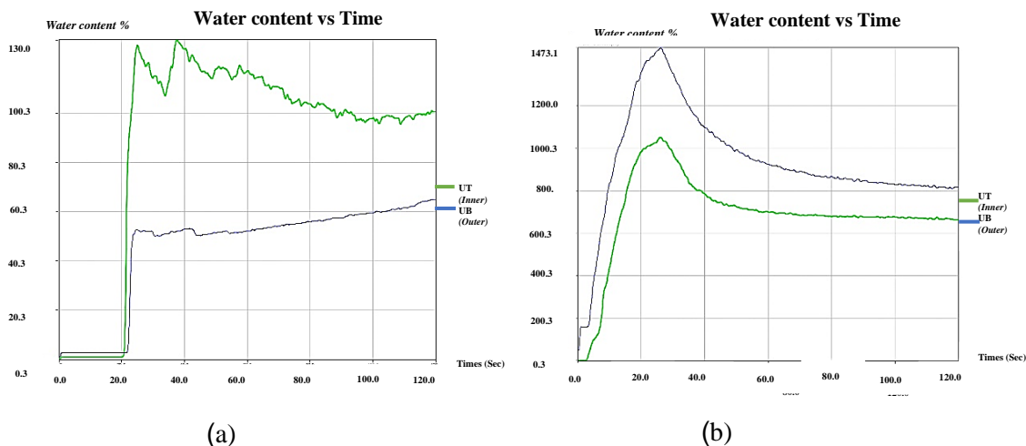
Figure 7 Sample (2) water content curves through 120 seconds a) drop water on the face of the fabric (Twill 1/3) polyester microfiber 75%:bleached cotton 25% 300/ 288 den, b) drop water on the back of the fabric(Twill 3/1) polyester microfiber 25%:bleached cotton 75% 300/ 288 den
