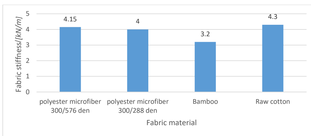
Figure 2 The effect of weft composition on the fabric stiffness
