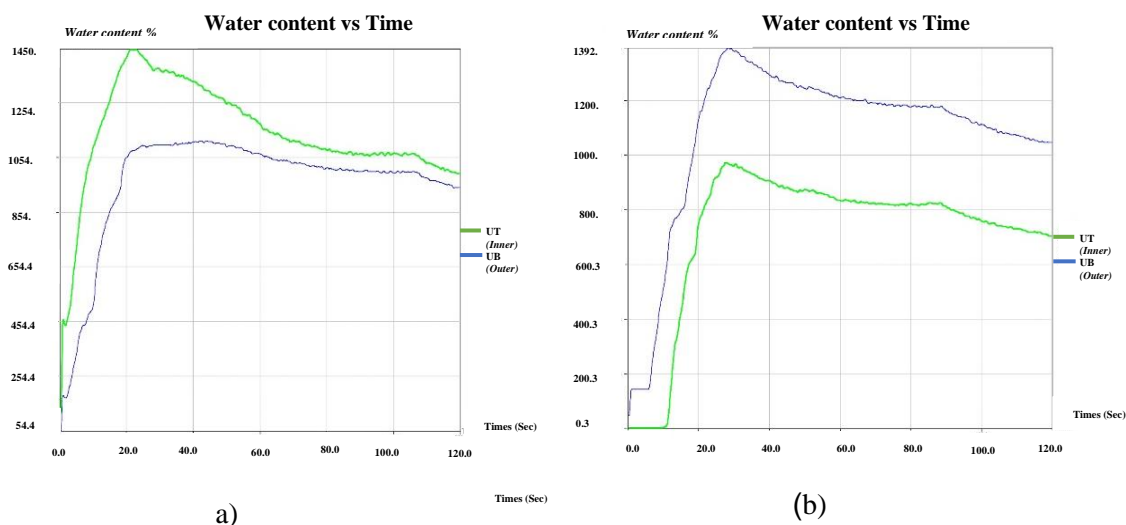
Figure 8 Sample (3) water content curves through 120 seconds a) drop water on the face of the fabric (Twill 1/3 Bamboo75%: bleached cotton 25%), b) drop water on the back of the fabric(Twill 3/1) Bamboo25%: bleached cotton 75%
