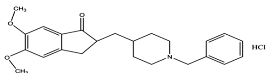
Figure 1: Structure of donepezil hydrochloride.
