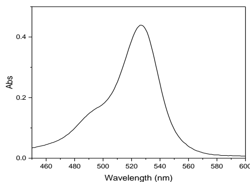
Figure 2: UV-Vis spectra of the ion-pair complex of (6.0 \mu\text{g/ml} ) of DNP and 1 \times 10^{-4} M EB dye
