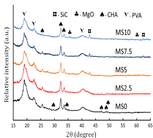
Fig. 4. XRD patterns of PVA/BHA/MgO/SiC of hot-pressed composites at 120 °C.
