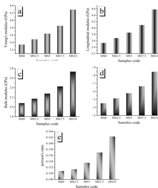
Fig. 10. a) Young's modulus, b) longitudinal modulus, c) bulk modulus, d) shear modulus, and e) Poisson's ratio for all hot-pressed samples.
