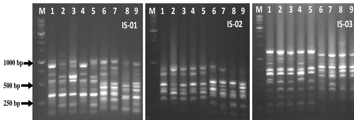
Fig. (4): PCR amplification profile generated with three ISSR primers from genomic DNA treated sorghum under study.
