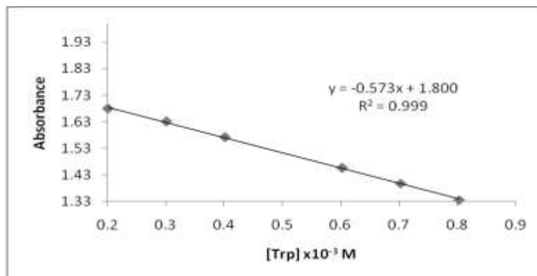
Fig. 6. Linear relation between absorbance –Trp concentration at \lambda_{\max} = 590 nm.
