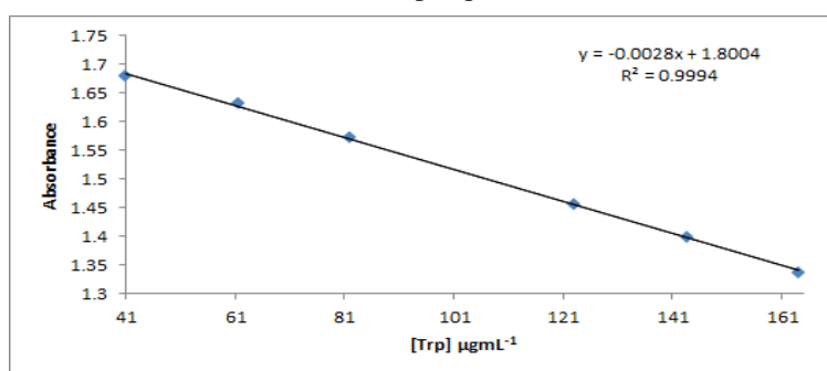
Fig.13. Calibration graph of the reaction between Trp and ferrioin (III).
