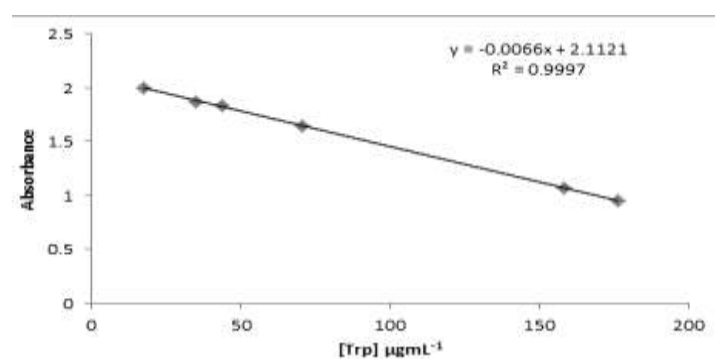
Fig. 15. Microdetermination of Trp in the synthetic mixture at \lambda_{\max} = 590 nm.
