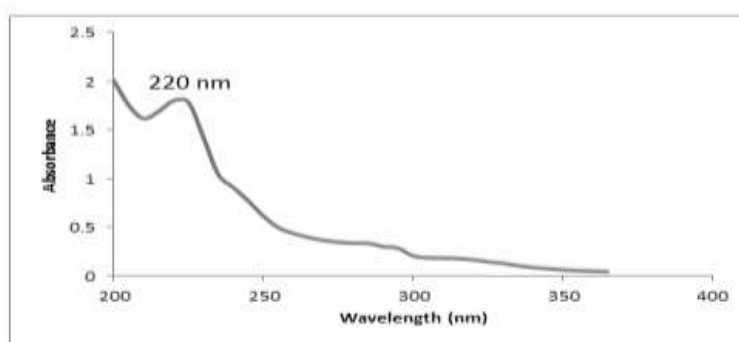
Fig. 12. Spectrum of 1.004 \times 10^{-4} M Trp in 0.3024 N \text{H}_2\text{SO}_4 medium.
