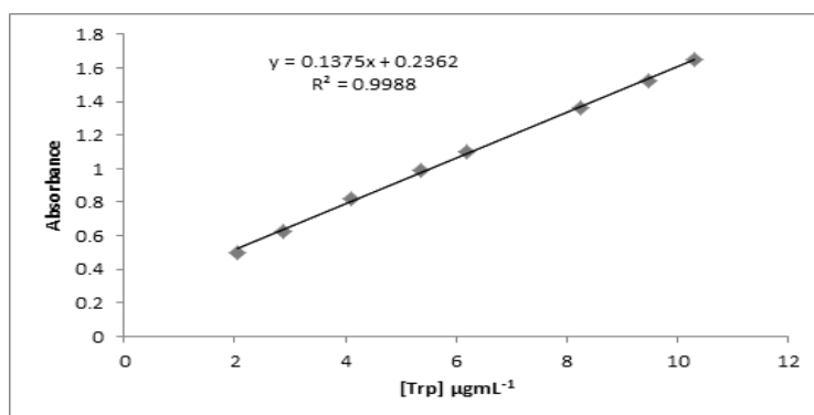
Fig.14. Calibration graph of the reaction between Trp in its oxidized form and Ferroin (II) at \lambda_{\max} = 515 \text{ nm} .
