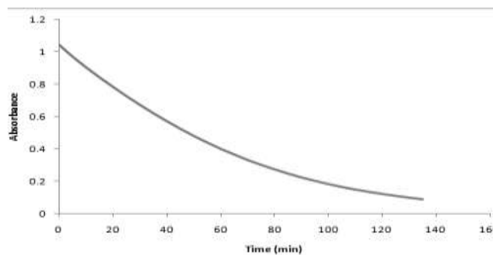
Fig. 9. Effect of time on the ion-pair formation between ferrioxalate (III) and Trp at \lambda_{\max} = 515 nm.
