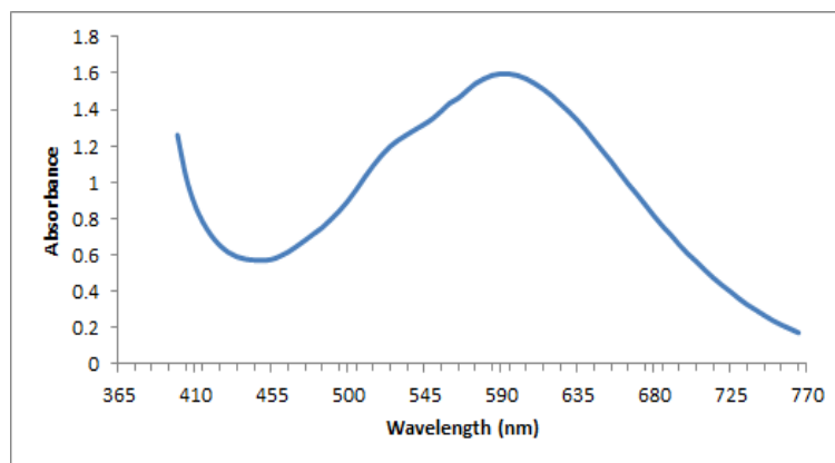
Fig.2. Absorption spectrum of ferroin solution (iron III sulfate complex) .
