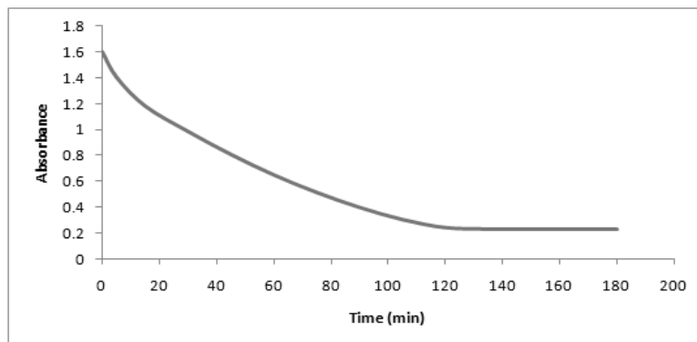
Fig. 3. Effect of time on the stability of the oxidized ferroin at \lambda_{\max} = 590 nm.
