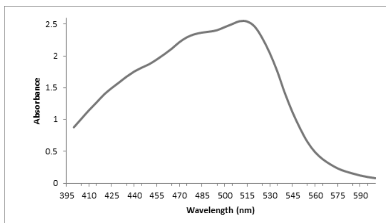
Fig. 1. Absorption spectrum of ferriin indicator solution.
