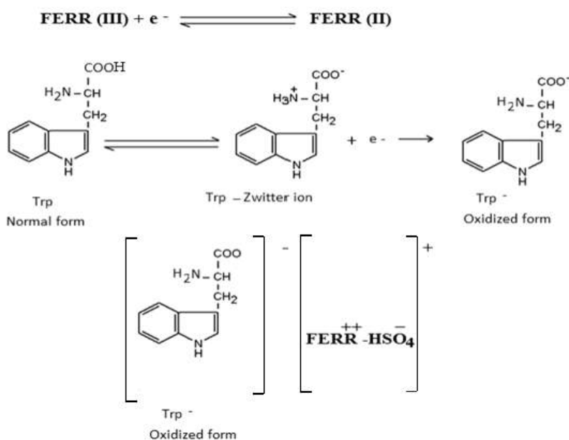
Scheme 1. Redox reaction of Trp-Ferriin (III).
