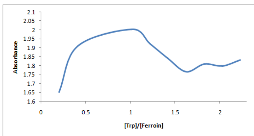
Fig. 8. Stoichiometric ratio of the reaction of ferriin (III) with Trp at \lambda_{\max} = 515 \text{ nm} using molar ratio method.
