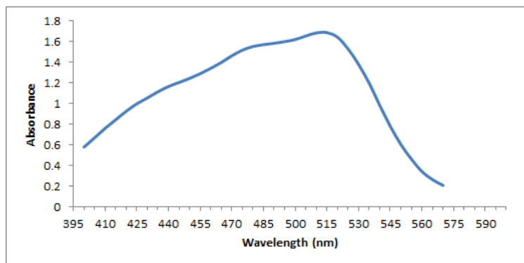
Fig. 5. Absorption spectrum of ferriin-Trp ion pair.
