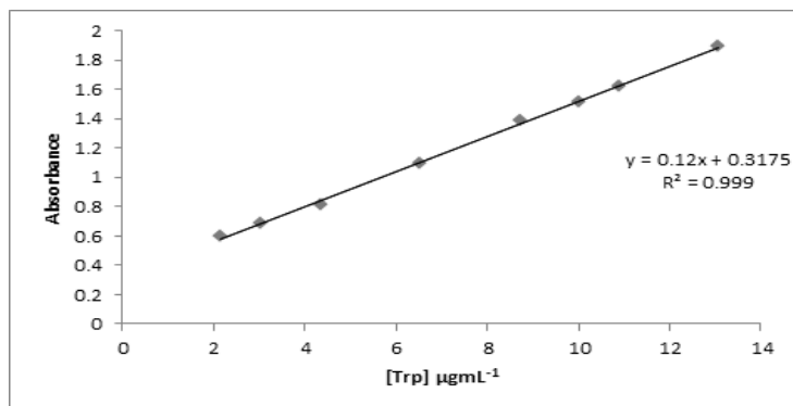
Fig.16. Calibration graph of Trp in the synthetic mixture using [ferroin III] = 2.0 \times 10^{-4} M at \lambda_{\text{max}} = 515 nm.
