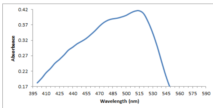
Fig. 4. Absorption spectrum of the oxidized ferroin solution after 3 hr from the beginning of the oxidation reaction.
