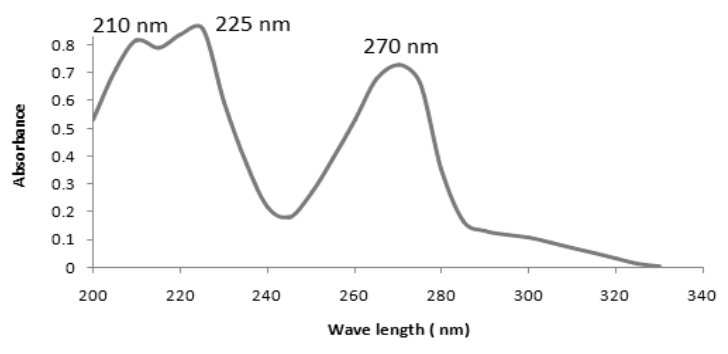
Fig. 10. The UV absorption spectrum of the ferrioxalate (II)-Trp oxidized form product ( 1 \times 10^{-5} M) at 135 min.
