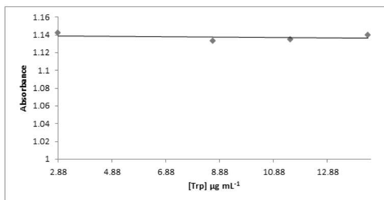
Fig. 7. The effect of variable [normal Trp] on the spectrum of ferriin (II)-Trp at \lambda_{\max} = 515 nm.
