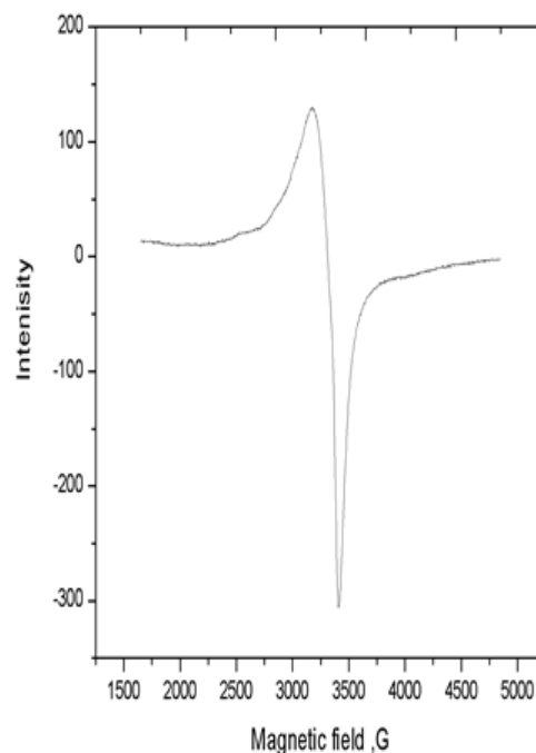
Fig. 2. ESR for [Cu (L)2] H2O complex.
