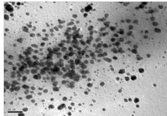
Fig.5a. TEM image of silver nanoparticles formed using 1.0 mM of AgNO 3 and 1.0 mL of Geotrichum candidum .
