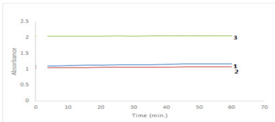
Fig 1. Effect of time on the ion pair reaction products of 1.FLZ-Rbeng, 2.VRZ-Rbeng, at \lambda_{\text{max}} = 575\text{nm} . 3. BTZ-Rbeng at \lambda_{\text{max}} = 580 nm.
