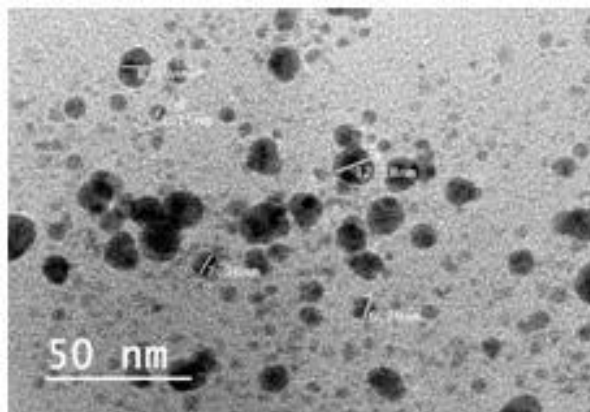
Fig. 1. (b): TEM image of SA/PVP hybrid emulsion loaded with TBHQ.
