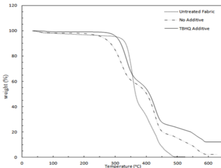
Fig. 2. TGA of untreated and water repellent fabric samples.
