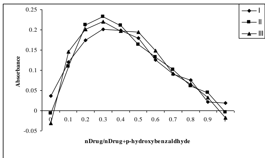
Fig. 3 a. Stoichiometric ratio of the reaction of p-hydroxybenzaldehyde with cited drugs using contentious variation method. [Drug]= 1 \times 10^{-3} M at \lambda_{\max} = 402 nm and T = 50^{\circ}\text{C} .
